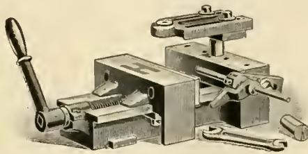
GRAHAM JIG VISE.
